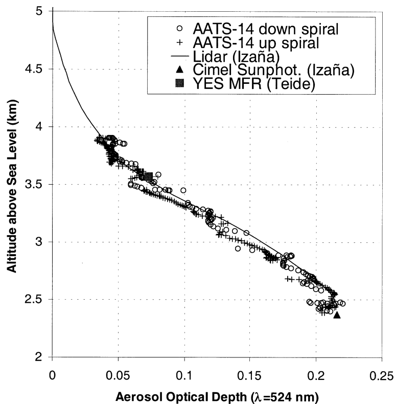
Fig. 20. AOD profiles from lidar ( \lambda = 524 nm) and AATS-14 ( \lambda = 524.8 nm) above Izaña. The lidar profile is constrained to match the Cimel AOD. Also shown the MFR AOD at nearby Teide at 3570 m a.s.l. (for Cimel and MFR the AODs are interpolated to \lambda = 524 nm).
