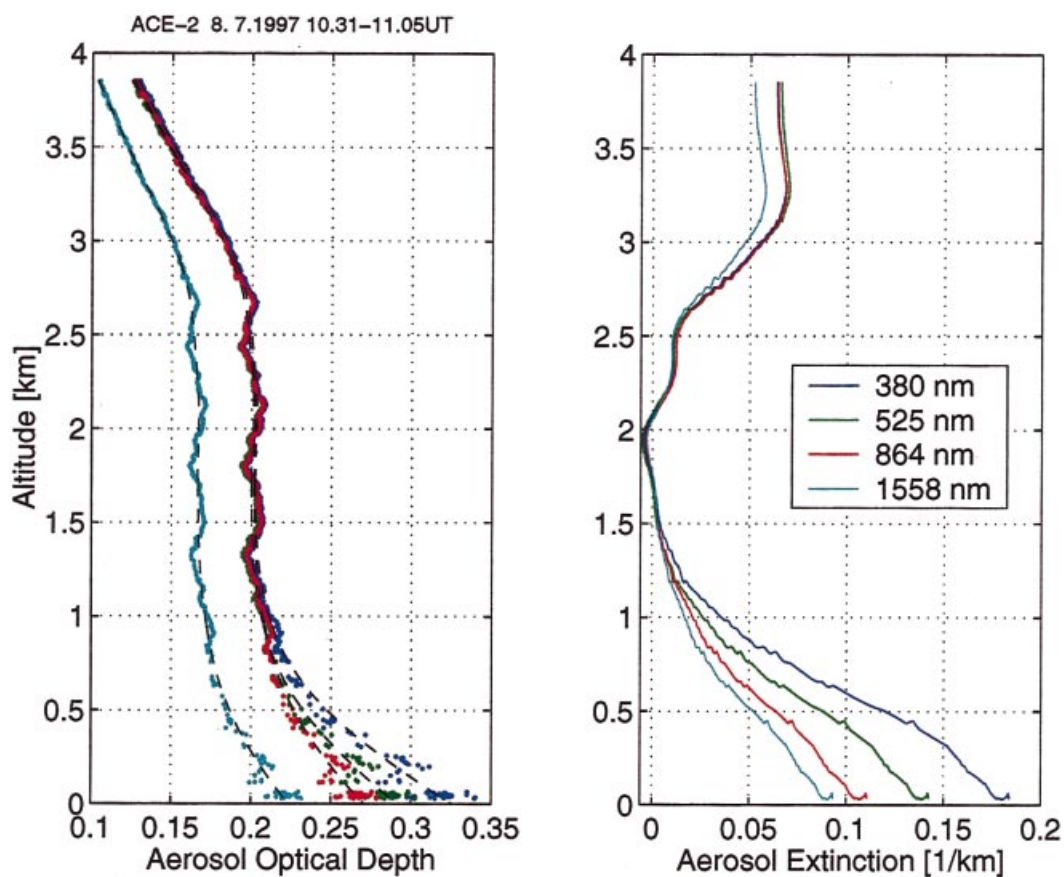
Fig. 2. Aerosol optical depth and extinction profile retrieved from AATS-14 measurements during Pelican flight 15 on 8 July 1997. Only 4 of 13 aerosol channels are shown. The dashed lines indicate the smoothed AOD profiles used to derive extinction.
